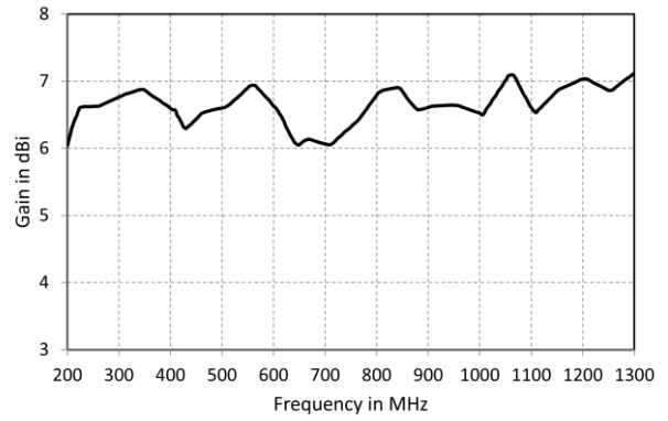
Fig. 2: Gain (typ.)
