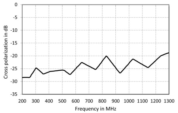
Fig. 4: Cross polarization (typ.)
