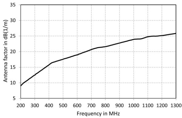
Fig. 3: Antenna factor (typ.)
